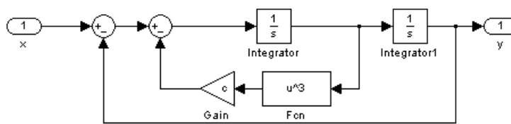
Figure 1.1 Block diagram in Simulink for equation 1.2
