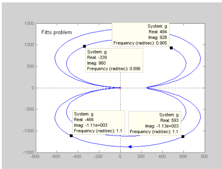
Figure 5.2 Nyquist plot for transfer function of equation (5.40)
