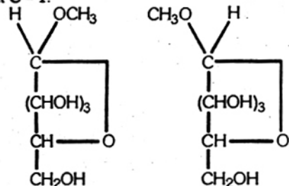
Methyl- \alpha -D-glucoside
