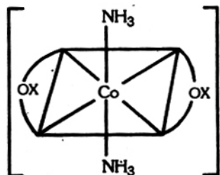
trans-isomer
