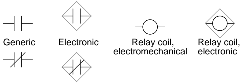
Relay components, "ladder logic" notation style
