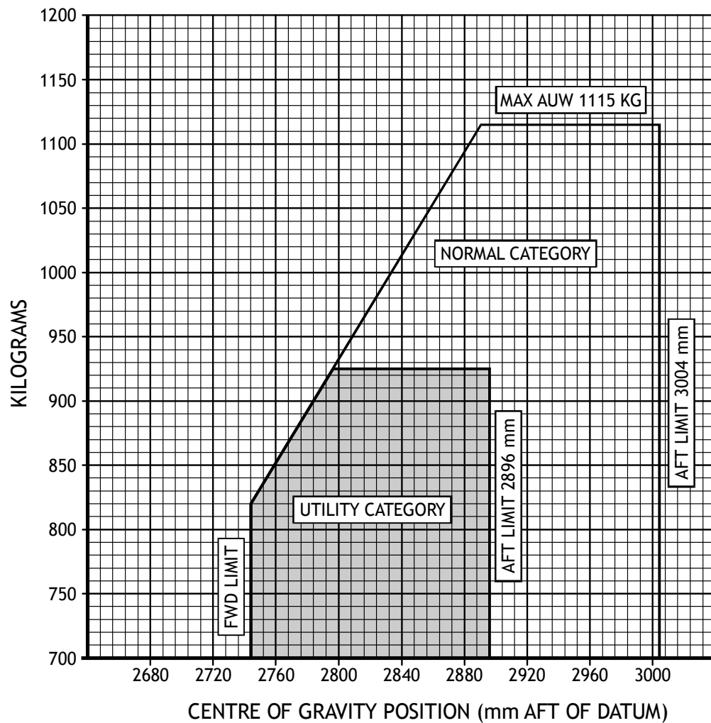
LOADING SYSTEM CHARLIE Figure 9
