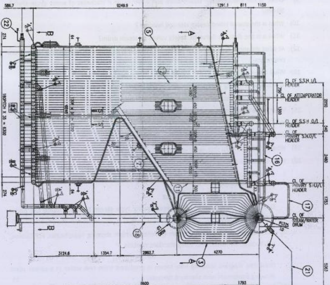
ELEVATION VIEW FROM BOILER RHS
